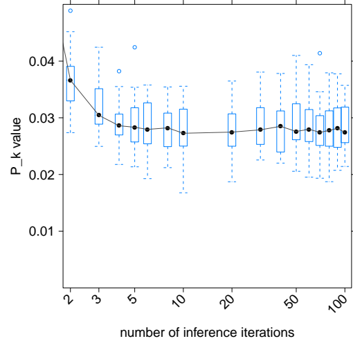
Figure 5: Figure of box plots for different inference iterations i and m = 1000 , T = 100 , \alpha = 50/T , \beta = 0.1 , r = 1 .
