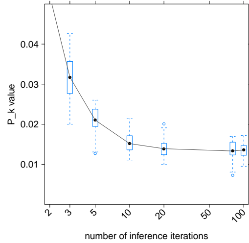
Figure 7: Box plot using the mode method d = true with several inference iterations i with m = 500 , T = 100 , \alpha = 50/T , \beta = 0.1 .
