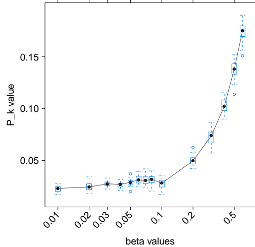
Figure 9: Box plot for several beta values \beta with m = 500 , i = 100 , T = 100 , \alpha = 50/T , r = 1 .
