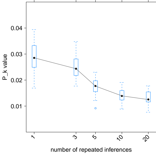
Figure 6: Box plot for several inference runs r , to assign the topics to a word with m = 1000 , i = 100 , T = 100 , \alpha = 50/T , \beta = 0.1 .
