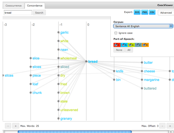
Figure 1: Screenshot of the Coocviewer application using the concordance view.
