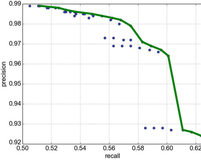
Fig. 1. Precision-recall plot of our matching method. Here we perform a grid search of two method parameters: profile similarity threshold \gamma \in [1; 4] and profile similarity ratio threshold \delta \in [3; 6] . The bold line denotes the best precision at a given recall.
