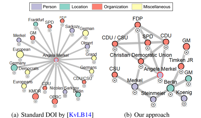
Figure 2: The DOI subgraph for the focus node “Angela Merkel”. a) The state-of-the-art approach by [KvLB14] results in a star-shaped subgraph hiding interesting structures and entities. b) Our approach shows a better structured subgraph.
