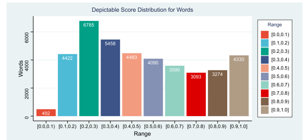
Figure 3: A bar chart of depictable score distribution for 40K English lemmas. We group tokens conditioned on the depictable scores into ten ranges, from [0.0, 0.1] to [0.9, 1.0]. This figure shows that around 10.84% of tokens whose depictable scores are over 0.9.
