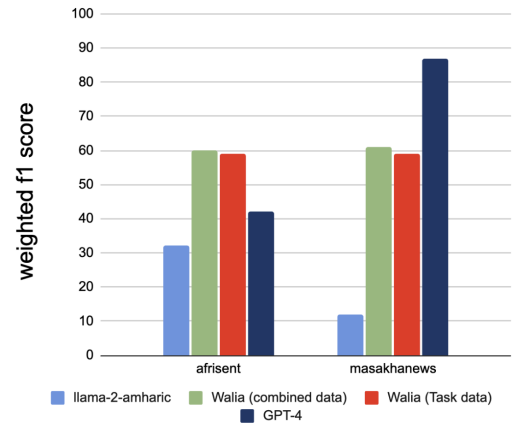
Figure 3: Generation scores: weighted f1 scores for AfriSenti and MasakhaNews (left) and SacreBLEU score for Amharic QA (right)
