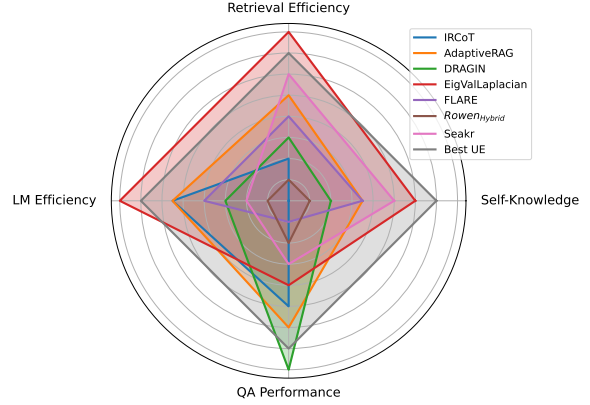
Figure 1: Performance comparison of the state-of-the-art models across efficiency metrics (number of LLM calls, Retrieval calls), QA quality metric (In-Accuracy), and the ability to identify self-knowledge (ROCAUC). The plot demonstrates the reverted ranks of the methods across 6 datasets.
