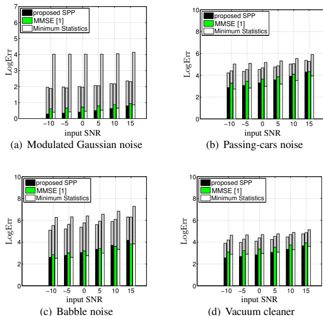
Figure 1: Comparison in terms of the LogErr for 320 TIMIT sentences and various input SNRs. The lower part of the bars represents the amount of noise power overestimation LogErrOver, while the upper part represents the noise underestimation LogErrUnder. The total height of the bars corresponds to LogErr.
