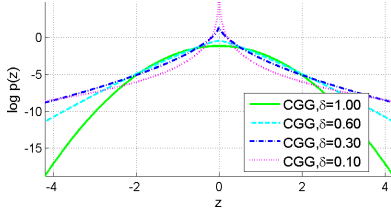
Fig. 1. Logarithm of the CGG prior (15) for different values of the shape parameter \delta and variance fixed to 1.
