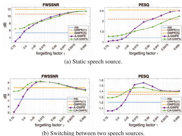
Fig. 1. Instrumental measures vs. forgetting factor \gamma for the considered experimental scenarios.
