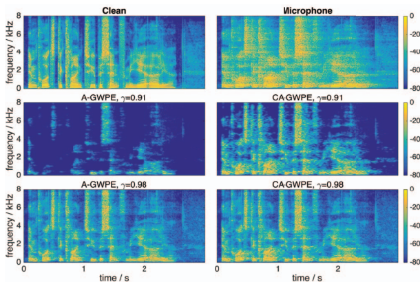
Fig. 2. Spectrograms of the clean speech signal and the microphone signal (top), and the output signals obtained using \gamma = 0.91 (middle) and \gamma = 0.98 (bottom).
